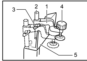
1. Vise arm 2. Vise rod 3. Screw 4. Vise knob 5. Guide fence
